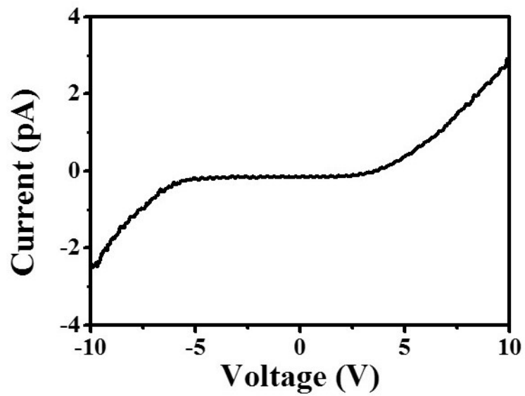
Fig. S1 The I - V curve of single SiC nanowire under the pressure of 0 nN in dark condition.
