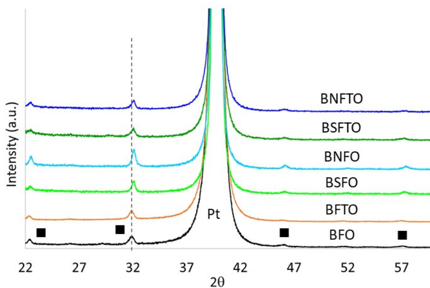
Figure S1. Normalised XRD patterns for the six compositions under study right after the crystallization of the films at 600°C/1h. Squares are assigned to the R_{3c} BiFeO 3 phase, while Pt stands for the platinum peak of the substrate. The grey dashed line around 2\theta = 32 shows the displacement of the peaks upon doping.
