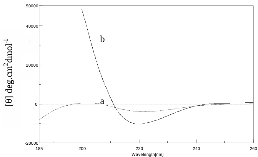
Figure: CD spectrum of peptide 1 in (a) in PBS, at pH 7.4 (b) in basic buffer, pH 10.6.
