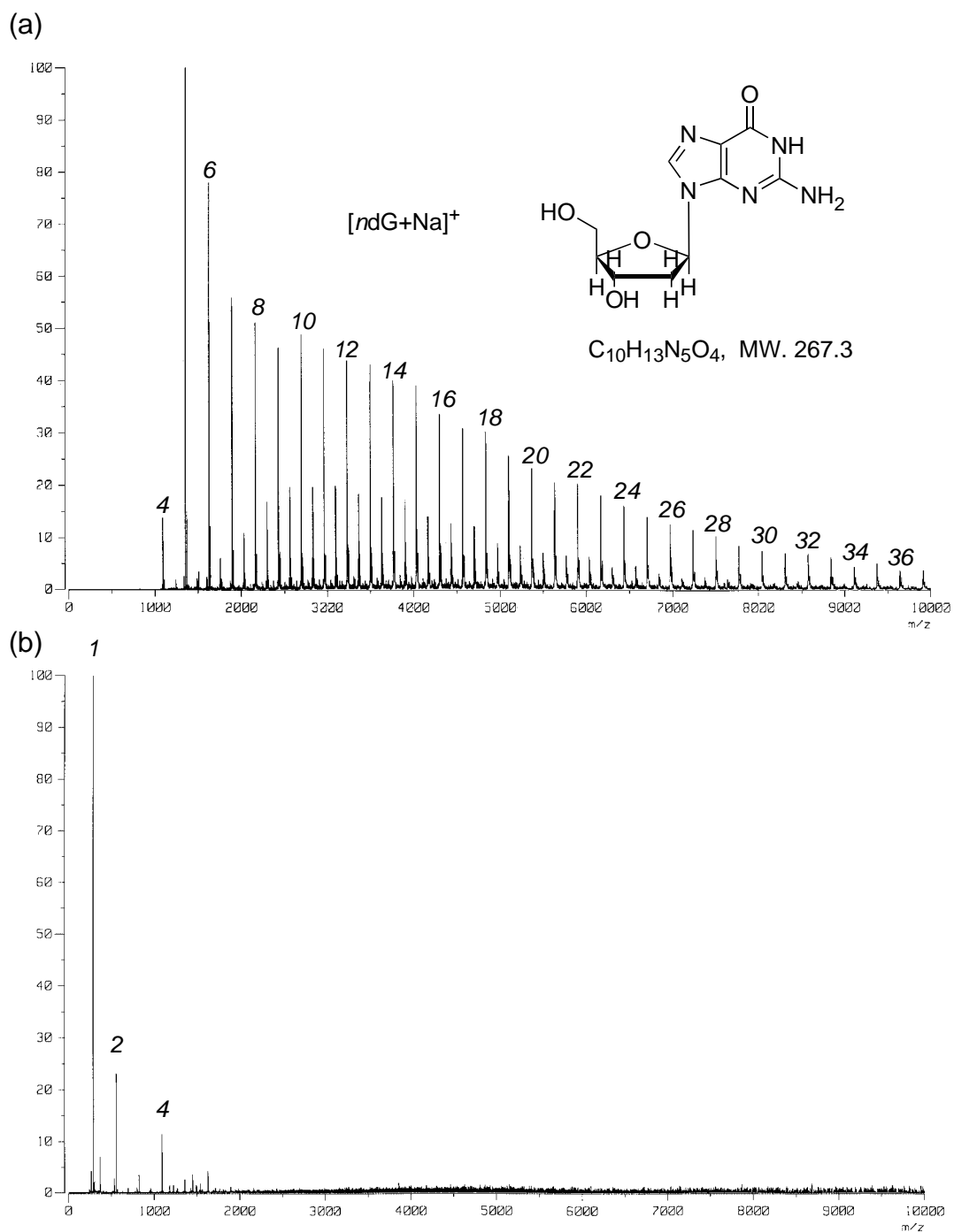
Figure S1 (a) CSI and (b) ESI-MS spectra of dG.
