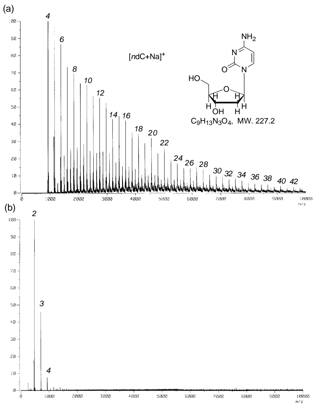
Figure S4 (a) CSI and (b) ESI-MS spectrum of dC.
