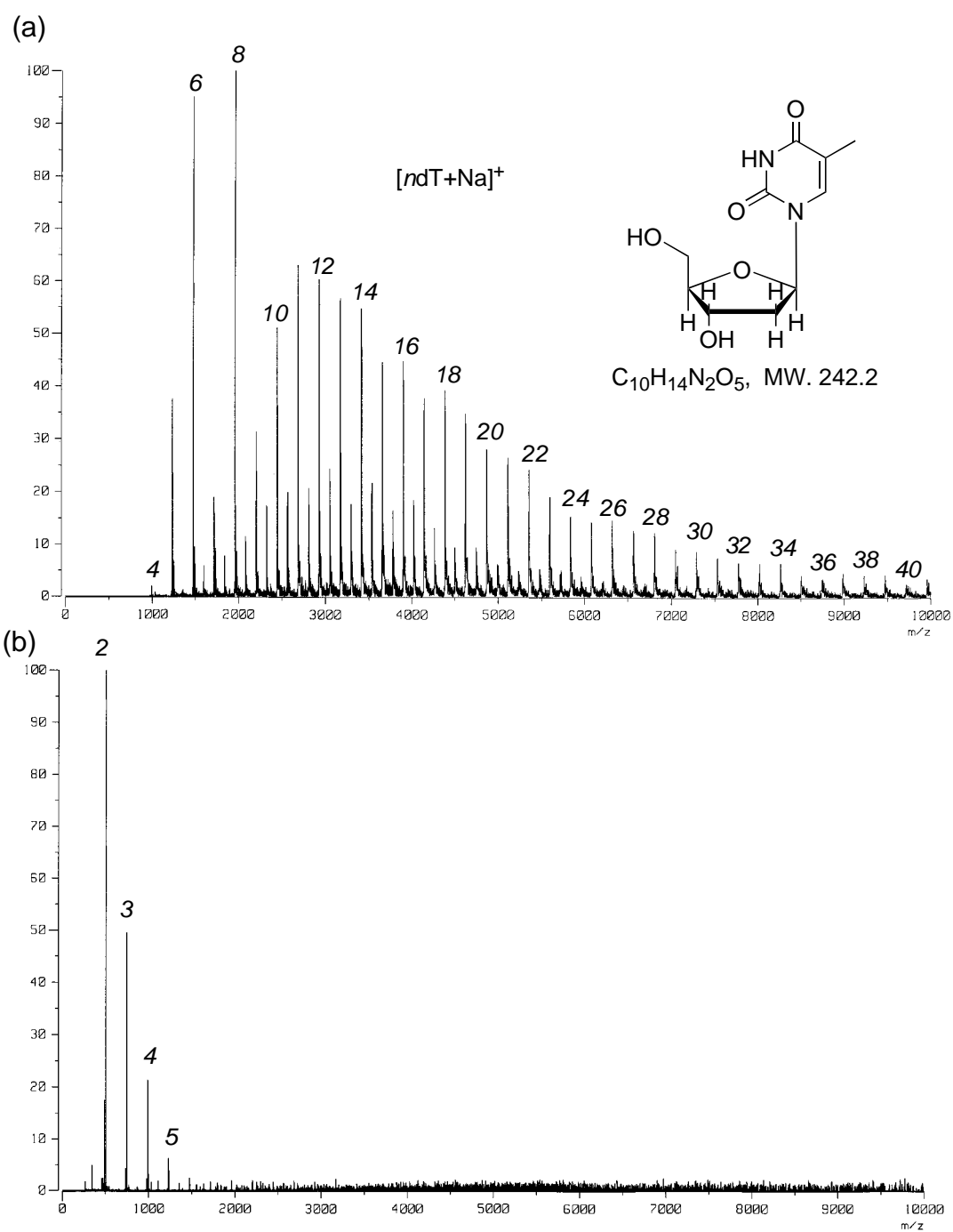
Figure S2 (a) CSI and (b) ESI-MS spectra of dT.
