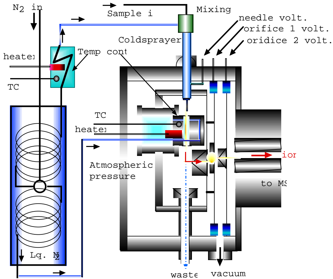
Figure S5. Schematic diagram of the coldspray ion source.
