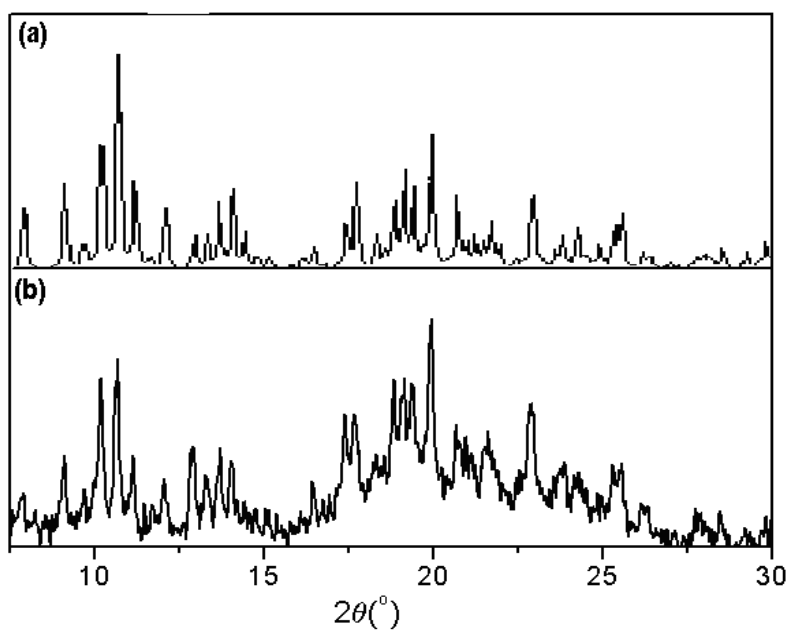
S2. The pattern calculated from the single-crystal data for complex 1 (a) and the powder X-ray diffraction pattern of the guest-lost samples 2 (b).
