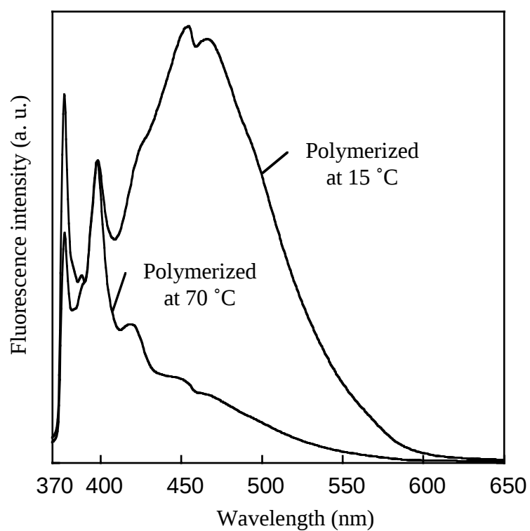
Fig. S-2 Fluorescence spectra of Pyr-lipid in the poly(methyl methacrylate) solid sheet.
