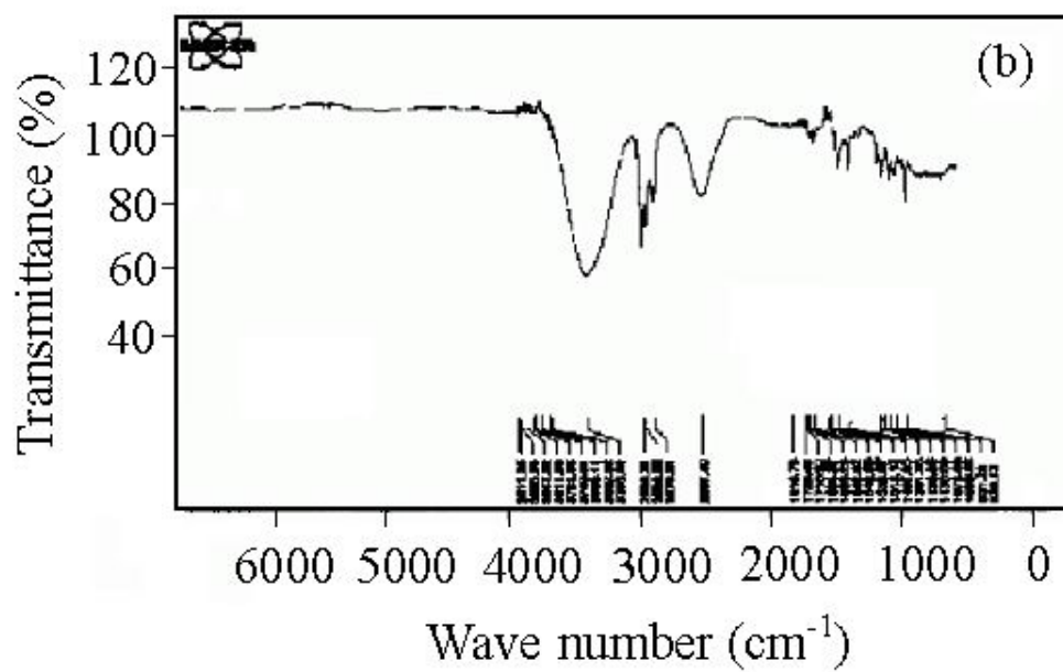
Fig. 1b Infrared (IR) spectrum of pure H 2 O (b): Measurement at 25°C, CaF crystal as lens, MCT Detector
