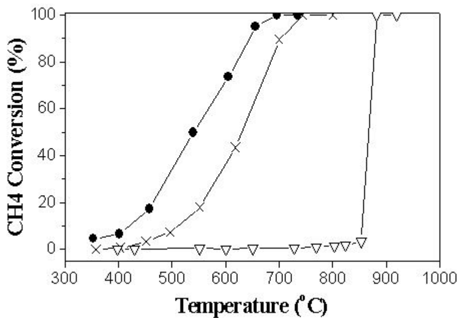
Fig. 6 The combustion activity over (●) \text{Ba}_{0.05}\text{La}_{0.95}\text{MnAl}_{11}\text{O}_{19-\alpha} catalysts prepared in the novel microemulsion. (×) \text{Ba}_{0.05}\text{La}_{0.95}\text{MnAl}_{11}\text{O}_{19-\alpha} catalyst prepared in the pure water. (▲) Quartz beads
