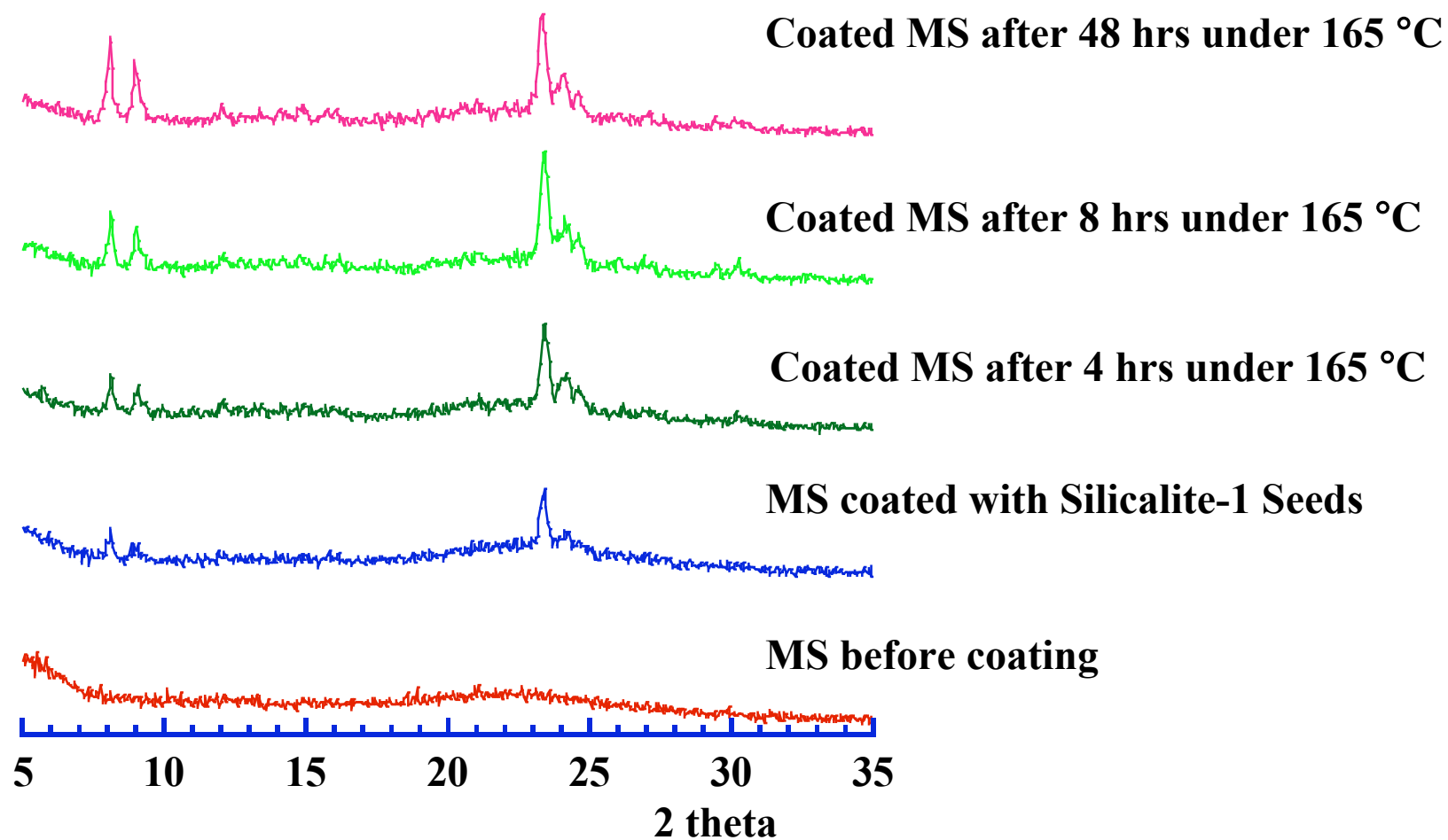
Figure S1. XRD patterns for mesoporous silica (MS) and MS coated with silicalite-1 during the hydrothermal synthesis procedure.
