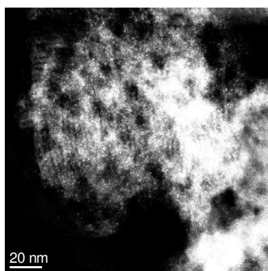
SI. 2 HAADF TEM image of gold nanoparticles supported on MCM-41 before reduction.
