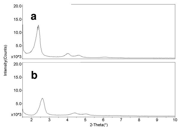
SI. 1 XRD patterns for mesoporous silica synthesized by a) batch method, MCM-41, b) aerosol method, aerosol silica.
