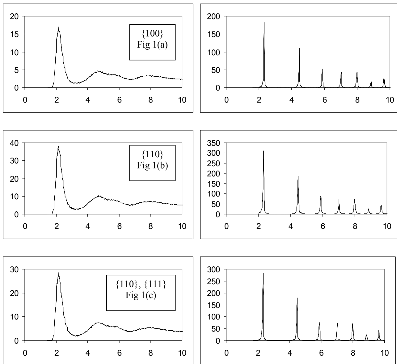
Fig. 1S Ce-O Radial Distribution Functions (RDF), calculated, left, for the amorphous configurations after 40ps and right the corresponding RDF for the final, 0K, configuration. Abscissa: Ce-O interatomic separation (Å); Ordinate: g(r) .
