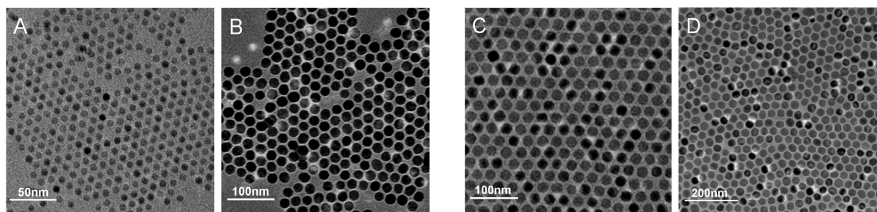
Figure 2 TEM photographs of magnetite nanocrystals with average diameters of 6.4 (A), 19.9 (B), 22.1 (C) and 28.6nm (D)
