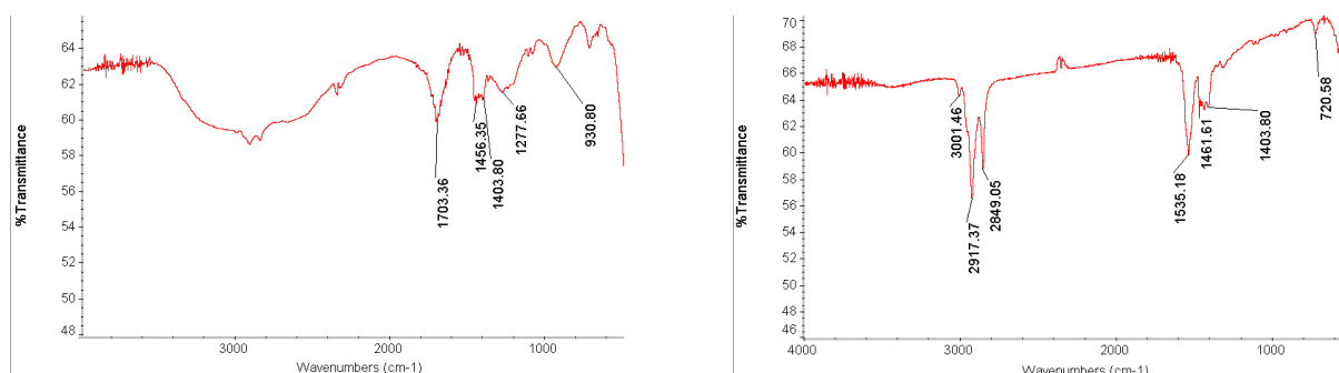
Figure 1 FTIR characterization of oleic acid (left) and iron oleate complex (right)
