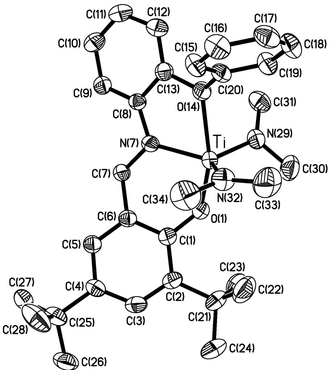
Figure S2 The molecular structure of 3b .
