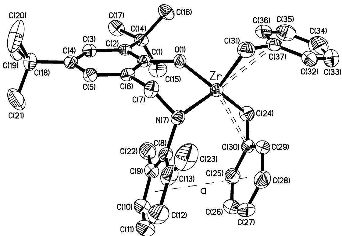
Figure S1 The molecular structure of 2 .
