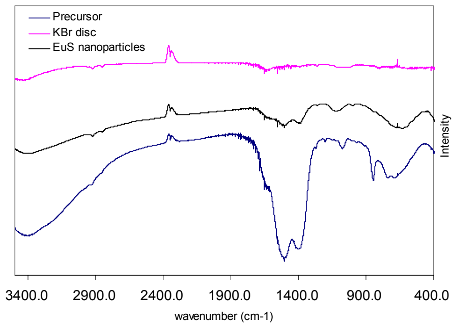
IR spectra of KBr disc, precursor and EuS nanoparticles.
