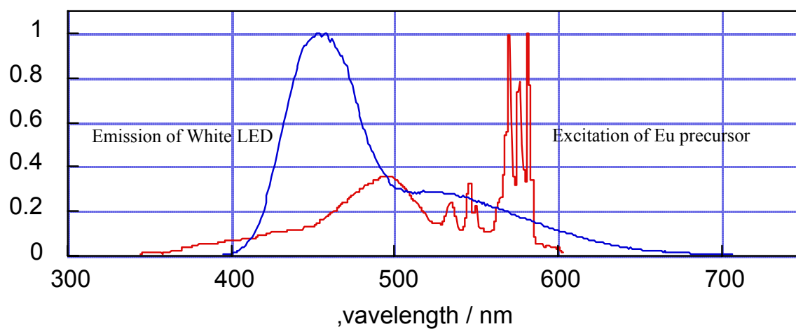
Spectra showing LED emission with an excitation spectrum of the precursor.
