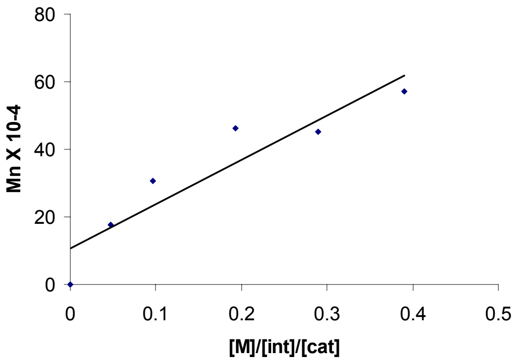
Dependence of Molecular Weight produced (GPC) on the ratio of Monomer to Initiator and Catalyst (after ref 33: D. Baskaran, Prog. Polym. Sci., 2003, 28, 521-581)
