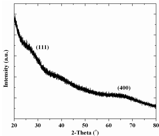
X-Ray diffraction spectrum of Ge NC powder. The diffraction peaks are diffuse due to the small particle size.
