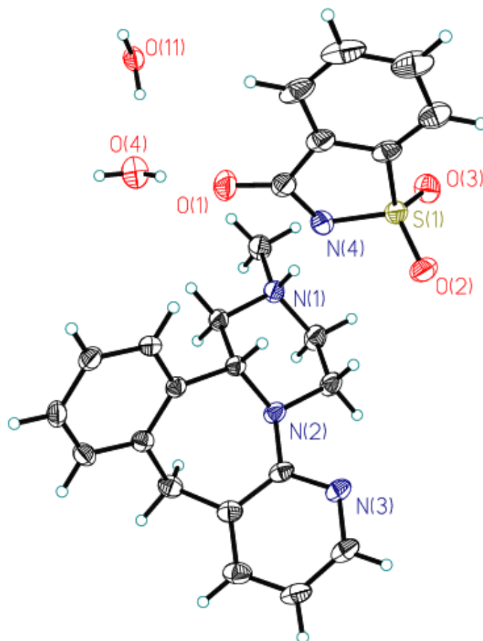
Fig.2 ORTEP diagram of mirtazapine saccharinate.
