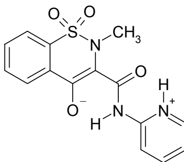
Piroxicam molecule as found in its saccharin adduct.
