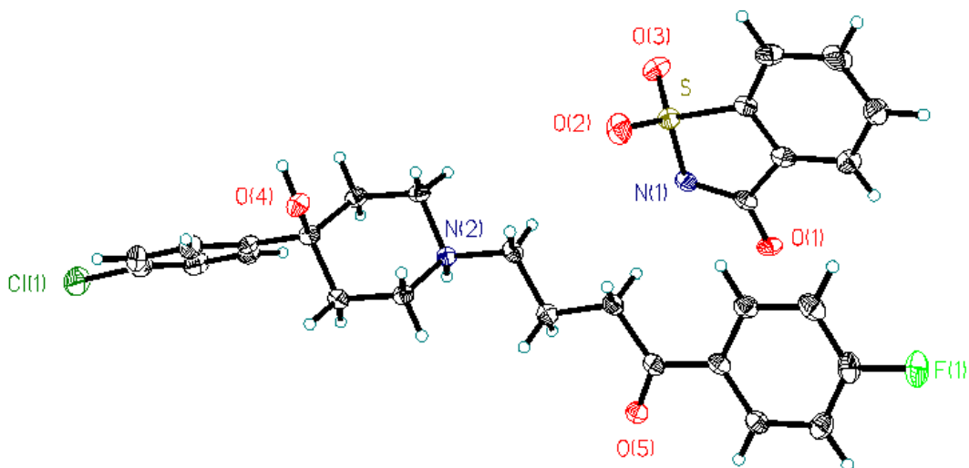
Fig.1 ORTEP diagram of haloperidol saccharinate.
