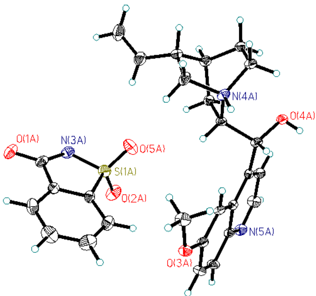
Fig.4 ORTEP diagram of quinine saccharinate.
