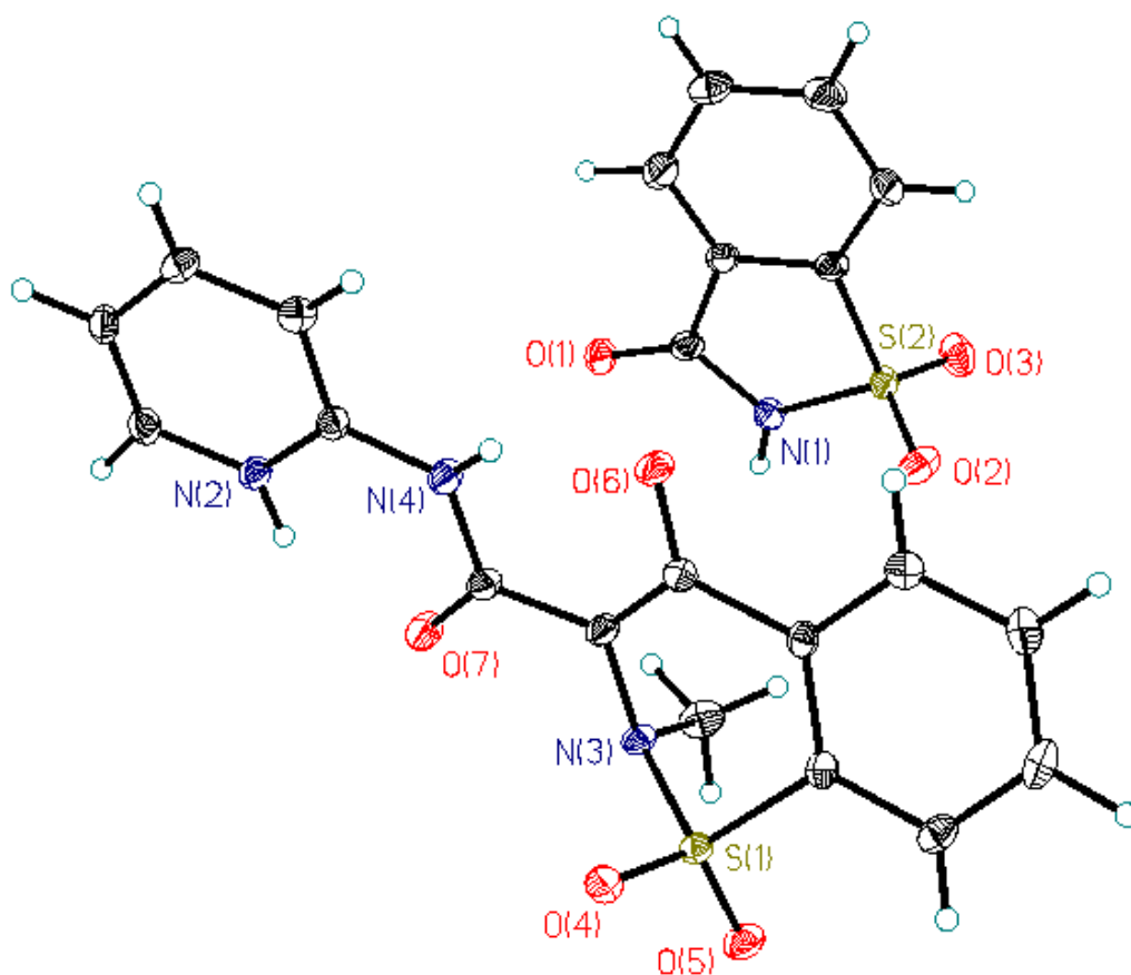
Fig.3 ORTEP diagram of piroxicam–saccharin.
