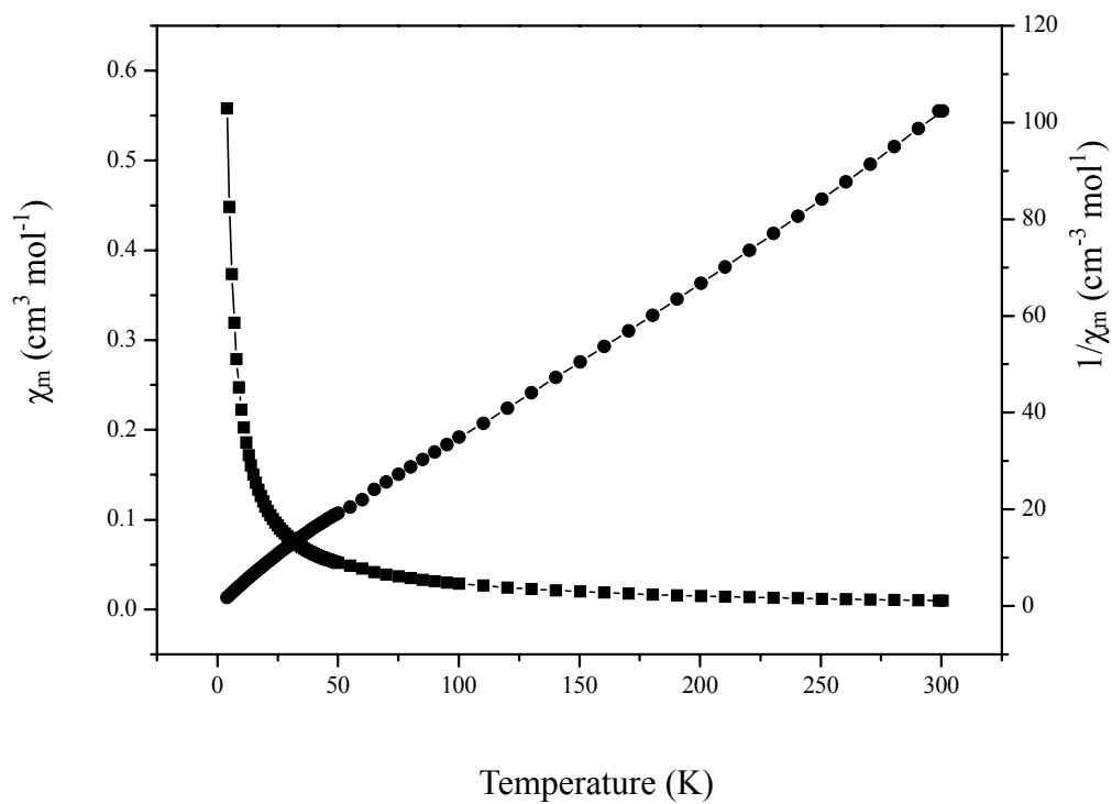
Figure S1. The \chi_m vs. T and the 1/\chi_m vs. T plots of \text{Co(PDC)(H}_2\text{O)}_2 \cdot (\text{H}_2\text{O}) .
