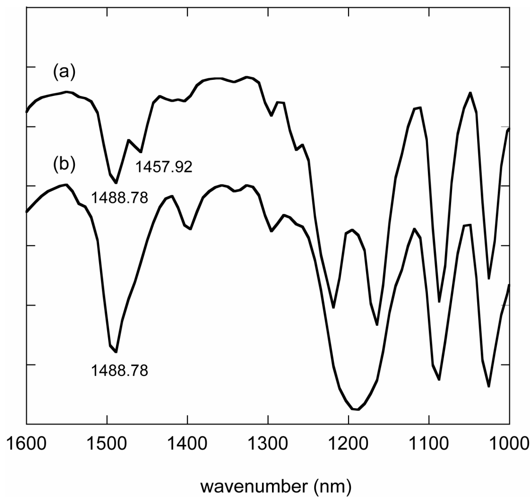
Figure S2. FT-IR spectrum of (a) Form I, 1 and (b) Form II, 4 in KBr
