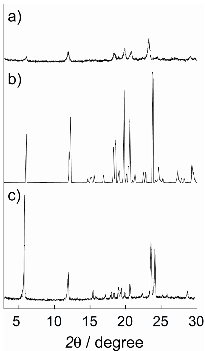
Figure S1. Powder X-ray diffraction profiles of a) 5 (crystal), b) 5 (simulated by TEXSAN) and c) 4 (crystal).
