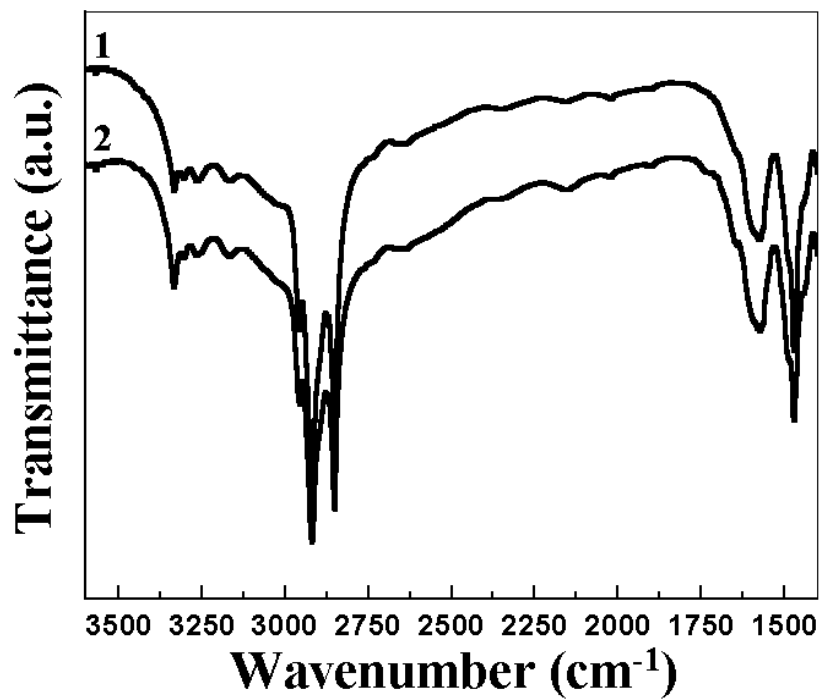
S1. FTIR spectra of ODA capped Ag nanoparticles before (curve 1) and after reaction with hydrophobized chloroaurate ions (curve 2)
