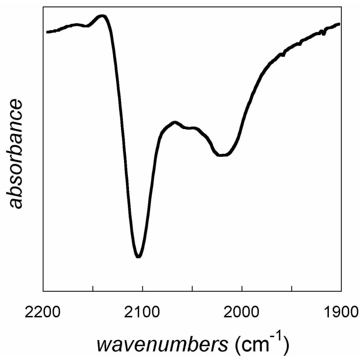
Figure S1. IR spectrum in the \nu_{\text{CN}} region for compound 2.
