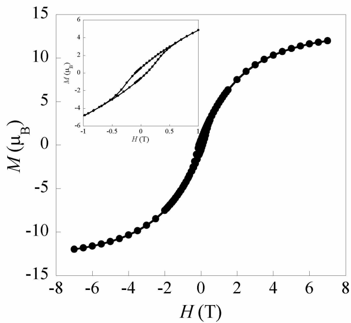
Figure S2. Plot of magnetization ( M ) versus field ( H ) for compound 2 at T = 2 K.
