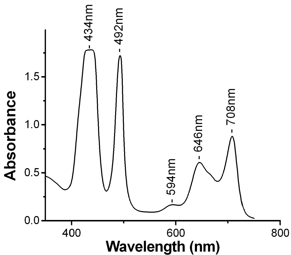
UV-vis spectrum of unmineralized J-aggregate nanofilaments at pH 2.
