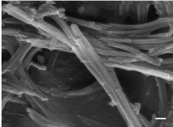
SEM image of calcined nanorods showing intact silica nanofilaments. Scale bar 100nm.
