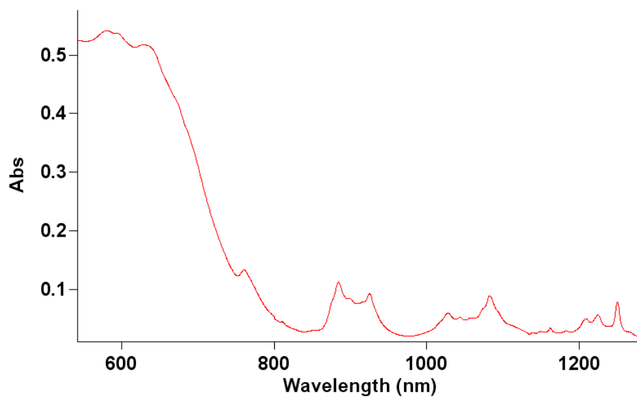
UVvis spectrum of 1
