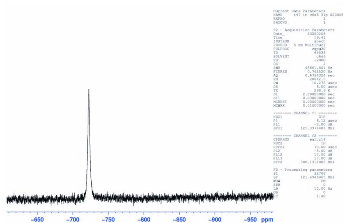
31P NMR spectrum of 2
