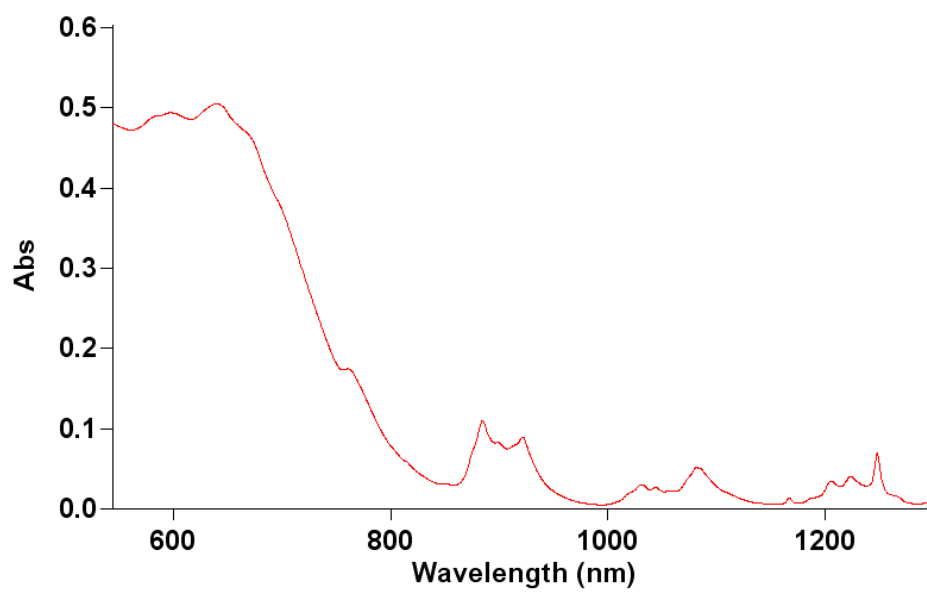
UVvis spectrum of 2
