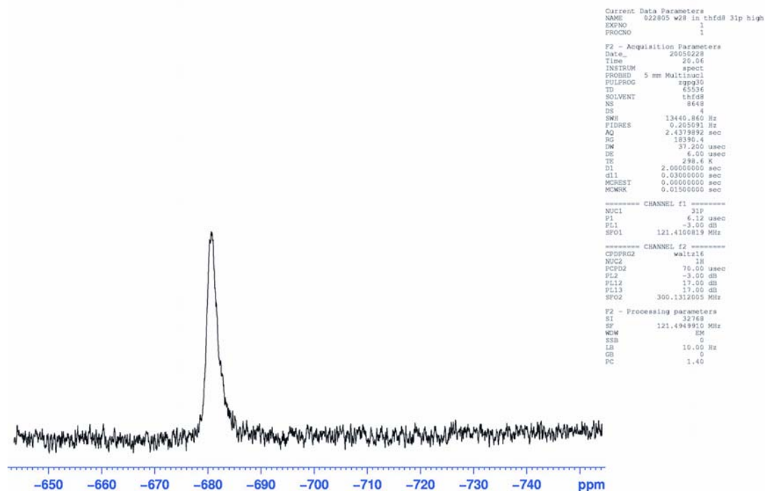
31P NMR spectrum of 1
