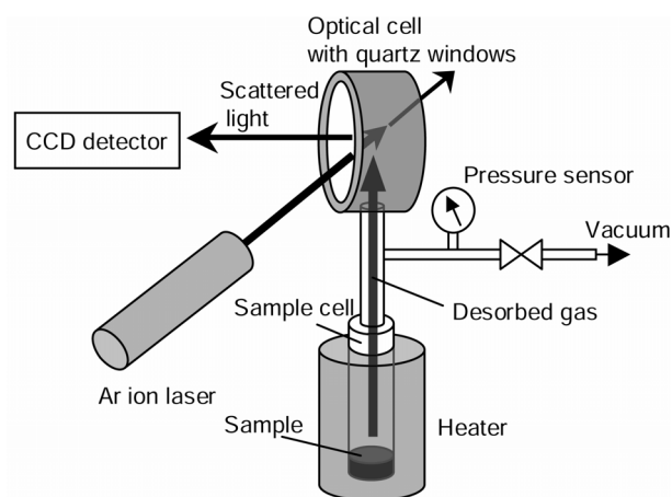
Fig. Schematic diagram of the apparatus.
