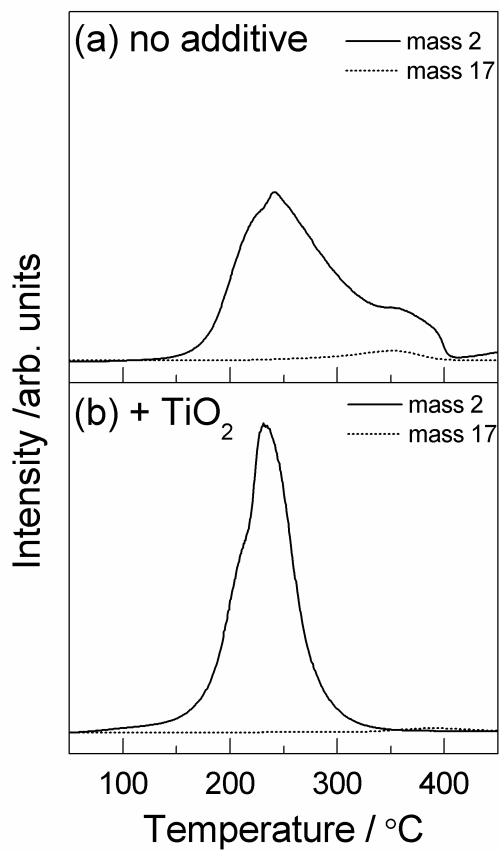
Fig. Thermal desorption mass spectra of (a) a mixture of 1:1 LiH + LiNH 2 and (b) the mixture with 1 mol% TiO 2 in the heating process up to 450 °C under a He gas flow atmosphere at a heating rate of 5 °C/min. Solid and dotted lines indicate mass 2 and mass 17, respectively.
