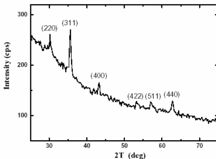
Figure S2. X-ray diffraction spectrum of Nafion/ \text{Fe}_3\text{O}_4 nanoparticles.
