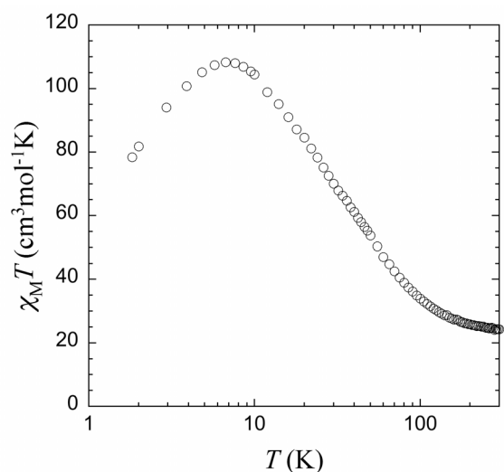
Fig. S1 Semilog plot of \chi_M T vs. T for complex 1 at 0.1 T.
