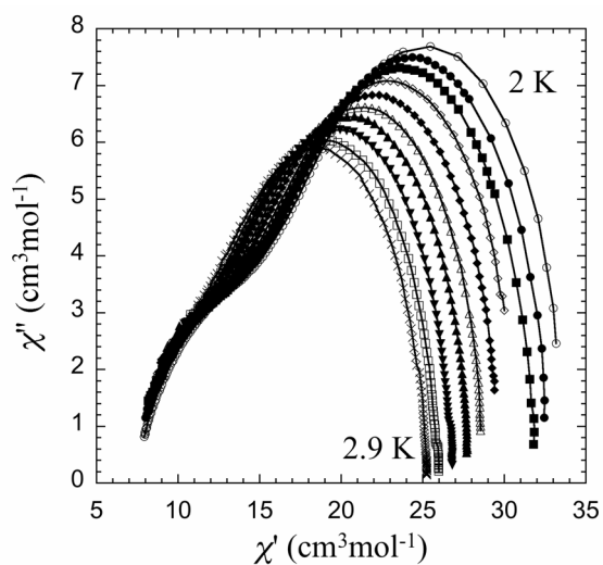
Fig. S2. Cole-Cole plots for complex 1 in the temperature range 2-2.9 K.
