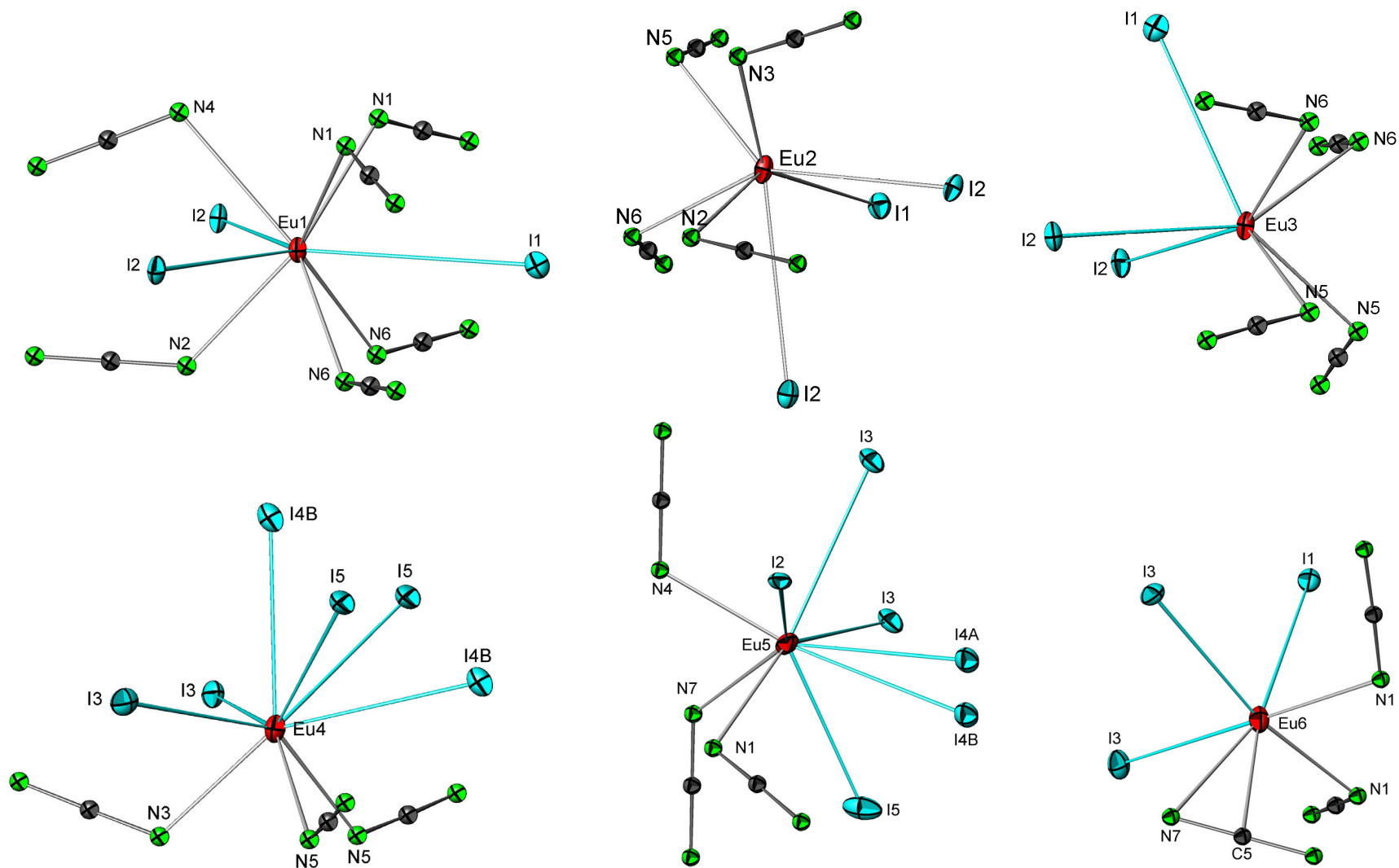
Supplementary Information: Coordinations of the six different Eu sites in \text{Eu}_8(\text{NCN})_{4.95}\text{I}_{6.10} .
