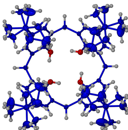
Ortep diagram of 2 . Notice the pentyl groups are disordered over two positions.
