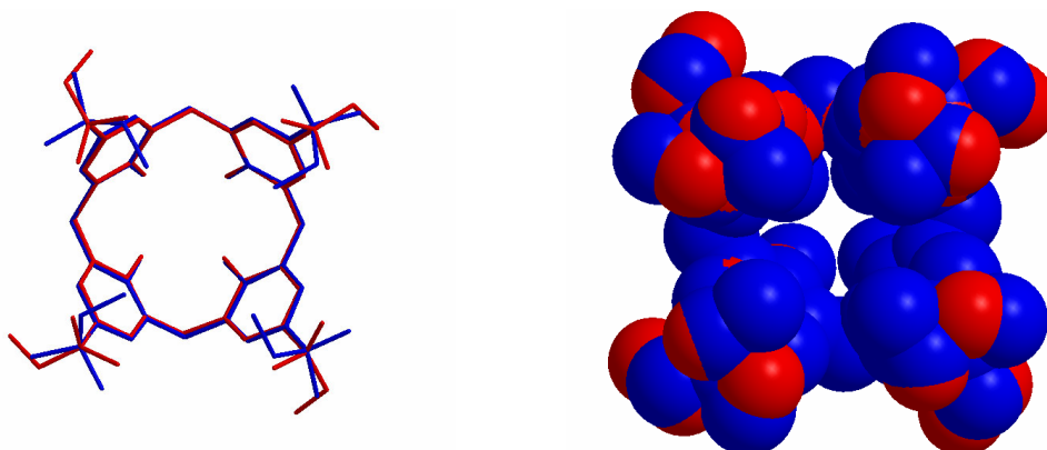
Overlay diagram of 2 and 2.toluene . Notice the tert -pentyl groups are pointing inside in 2 (Blue) whereas outwards in 2.toluene (Red)
