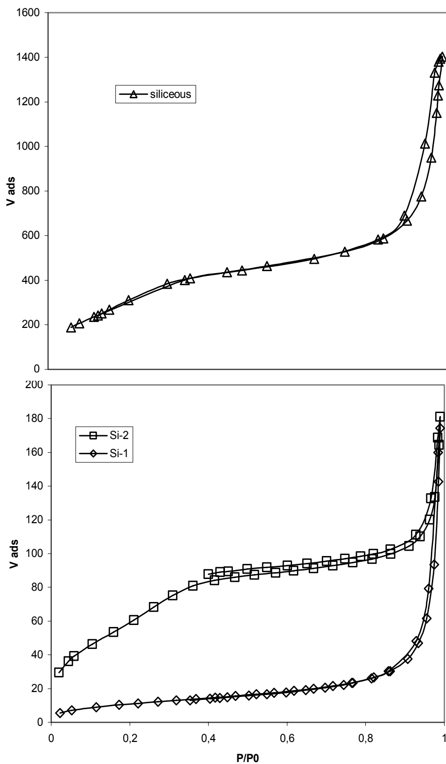
Figure 1. N 2 adsorption-desorption isotherms
