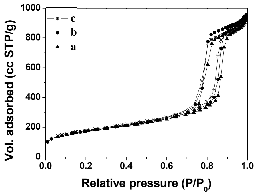
Fig. S1 N 2 adsorption-desorption isotherms of the samples prepared with a) C 6 ; b) C 7 ; c) C 9 .
