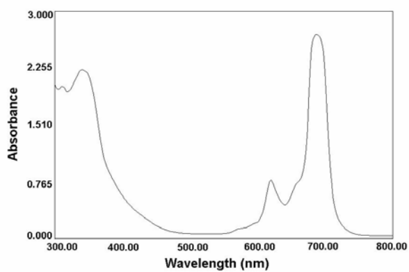
Fig. 1 Absorption spectrum of 2 in chloroform.
