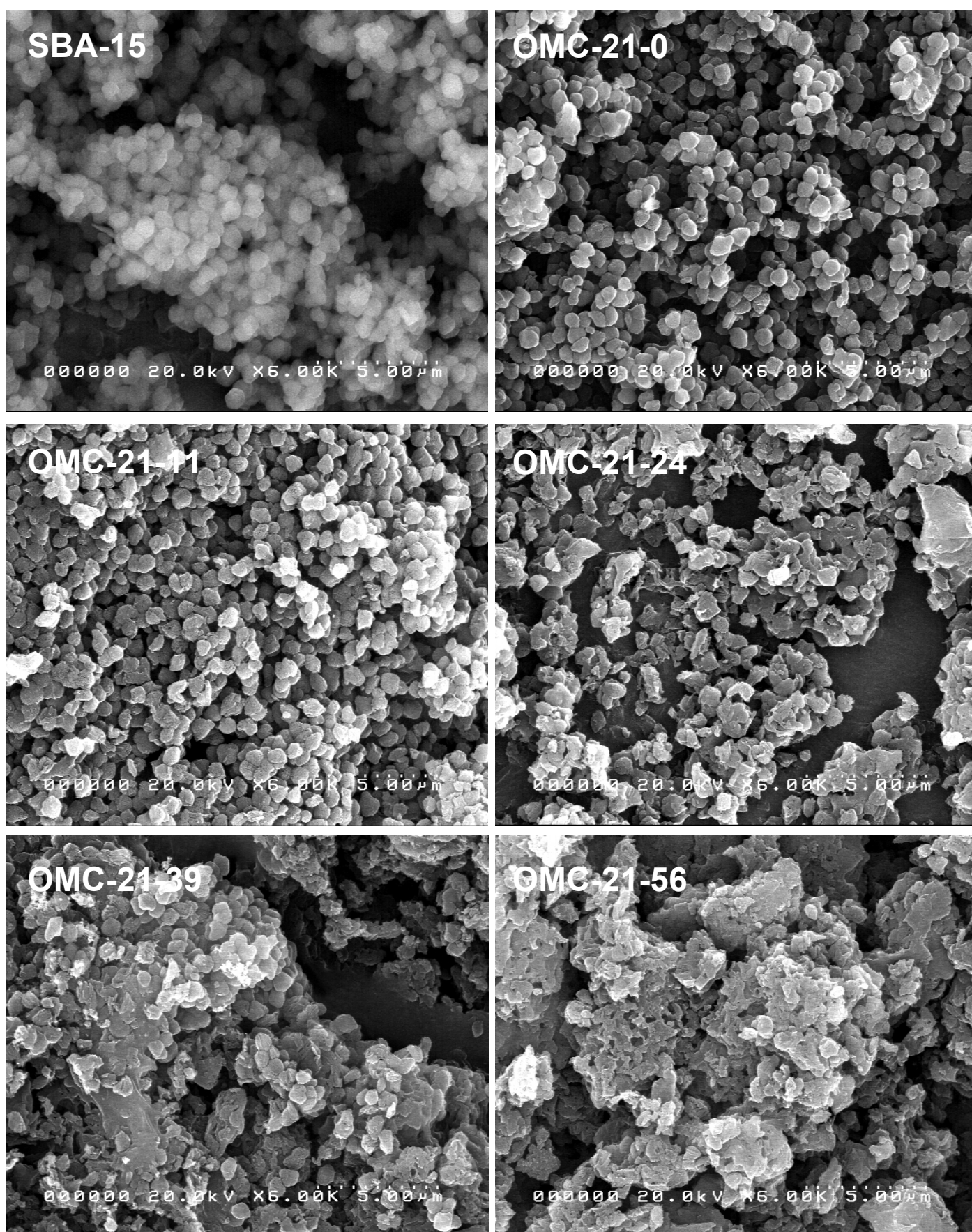
Fig. S3 SEM images with low magnification for the SBA-15 and OCM-21-y materials.
