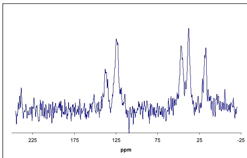
Figure S3. 13 C NMR spectrum of SIZ-6
