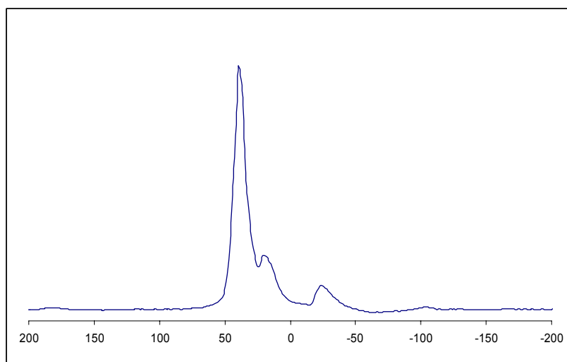
Figure S1. ^{27}\text{Al} MAS NMR spectrum of SIZ-6
