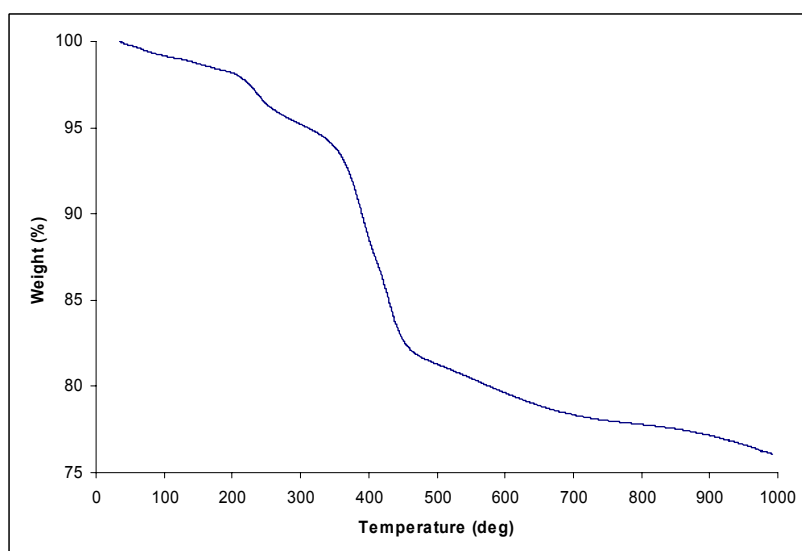
Figure S4 TGA of SIZ-6
