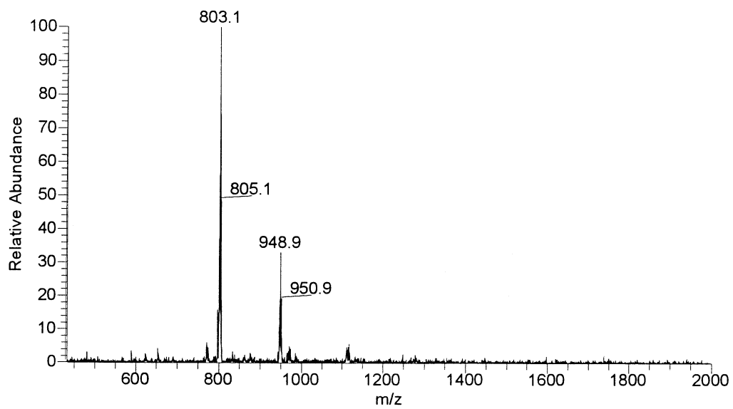
Figure S1. ESI-MS spectrum of the complex 1 in methanol solution
