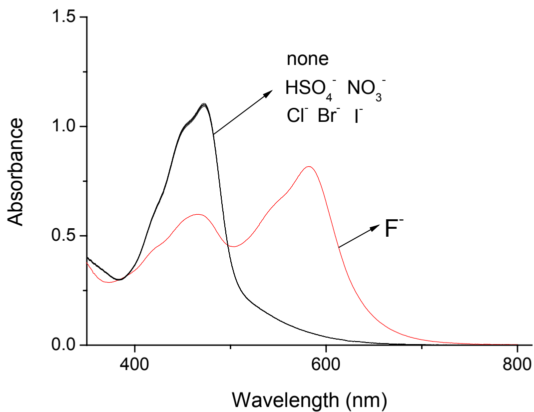
Figure S2. Uv-vis spectra of the complex 1 in MeCN ( 2.5 \times 10^{-5} M ) upon addition of one equivalent of anions as TBA + salts
