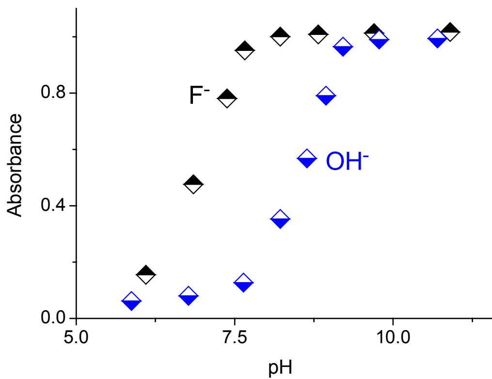
Figure S3 UV/ vis -pH titration curves at 580nm of 1 in MeCN ( 2.5 \times 10^{-5} M) upon addition of F - (black) and OH - (blue), respectively.
