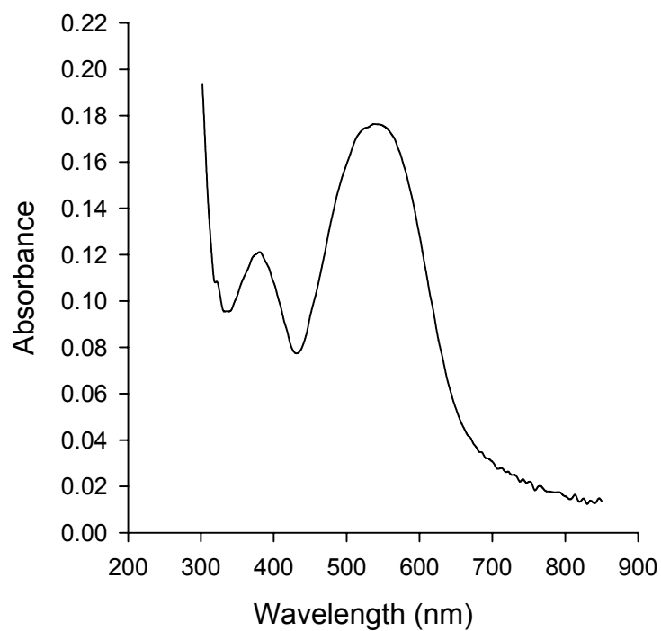
Electronic absorption spectrum of a film of 1 evaporated on glass
