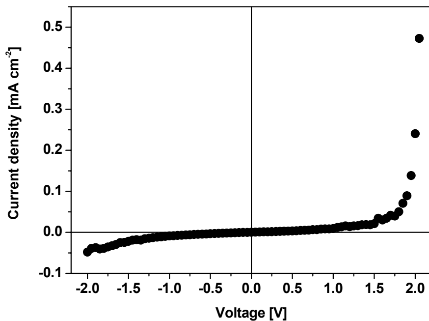
Current voltage curve of the cell ITO/1(25nm)/C 60 (25nm)/Al(60nm)
