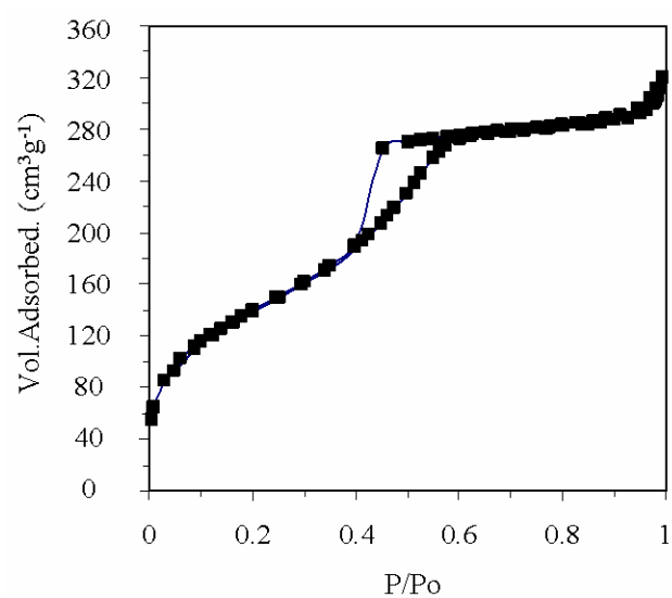
Fig. S Nitrogen adsorption/desorption isotherm of concomitantly prepared powder samples.
