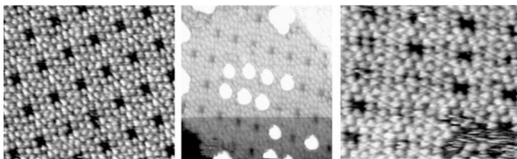
Electronic Supplementary Information (ESI): The STM data showing the nanocavities upon the thermal releasing of the guest species (cystine, C 60 and Phe-Phe, from left to right, respectively).
