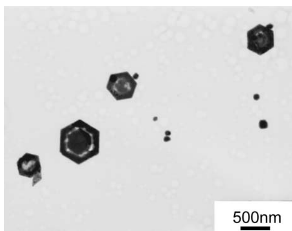
Fig. S3 TEM image of \text{PbF}_2 nanoplates with hole in the center synthesized by ultrasonic irradiation
