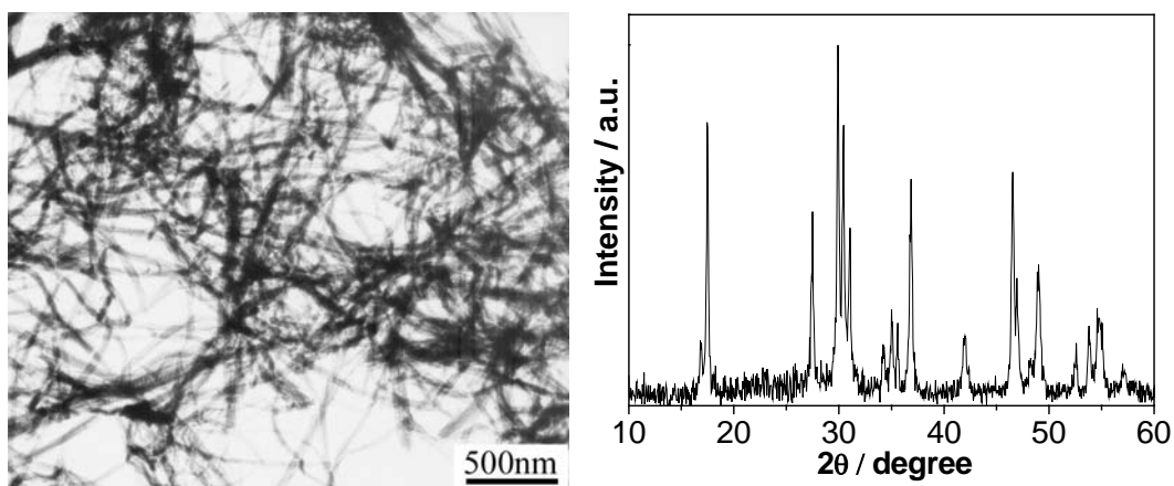
Fig. S1 TEM image and XRD pattern of the \text{Cd}(\text{OH})_2 nanowire byproduct
