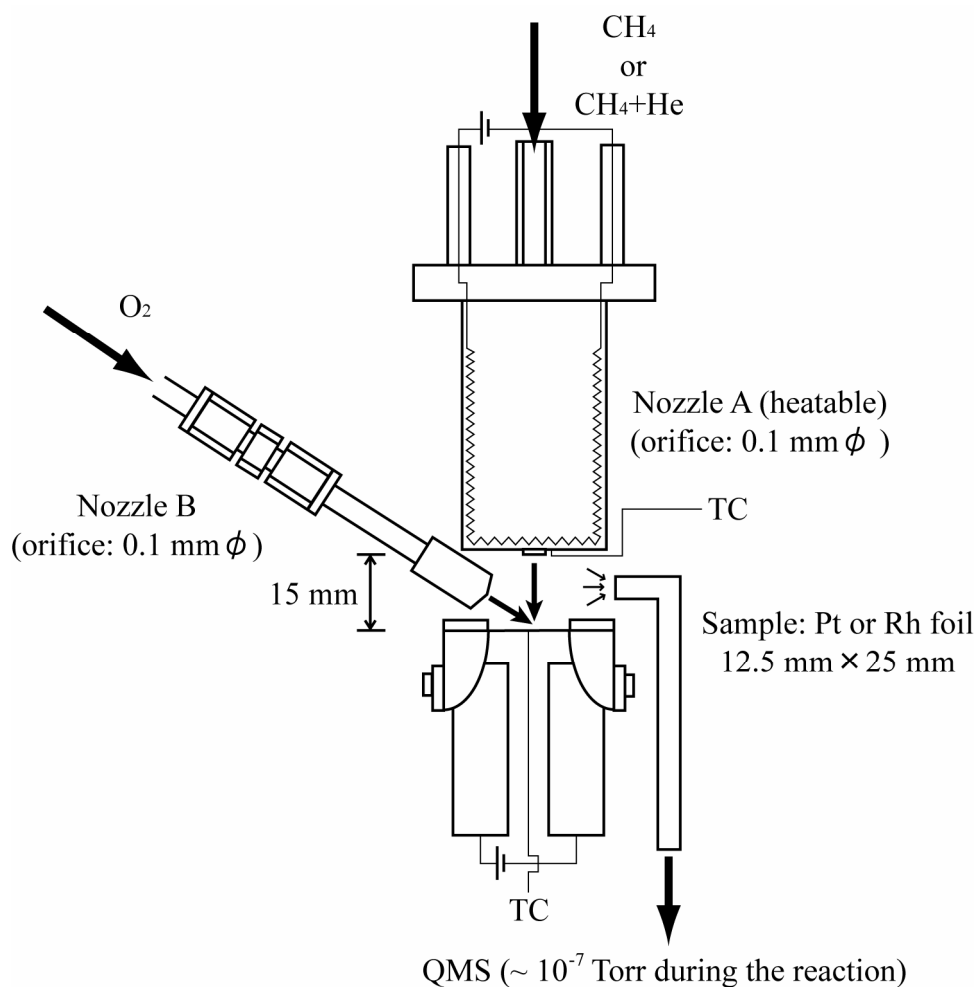
Figure Schematic diagram of a molecular-beam reaction apparatus. The background pressure in the QMS chamber reaches 5 \times 10^{-9} Torr.
