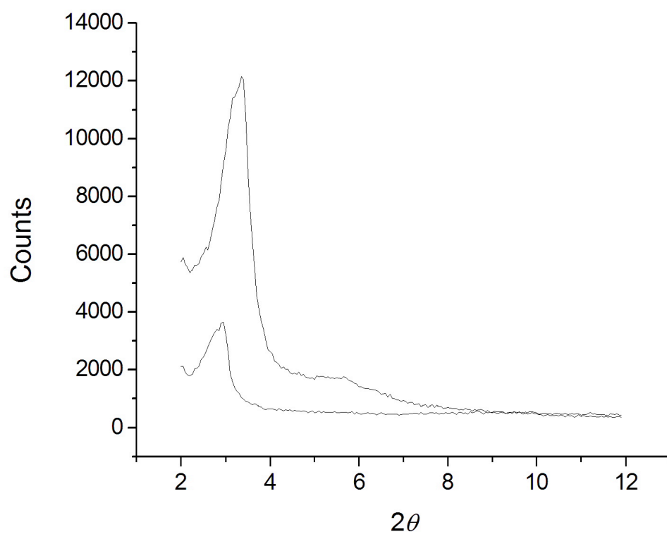
Fig. S1 X-Ray diffraction pattern for the silicate containing PdAu nanoparticles. The upper diffraction pattern belongs to the calcined sample, while the lower pattern is from the as-synthesised material.
