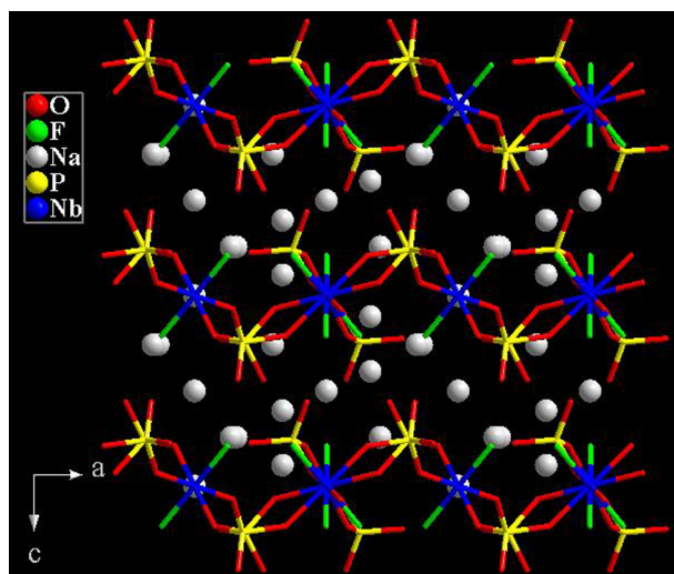
Fig. S1. View of the packing structure of 1 along the b -axis.
