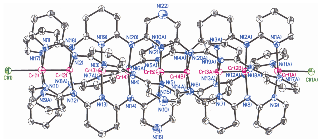
Fig. 1S The molecular structure of [\text{Cr}_9(\mu_9\text{-N}_9\text{-mpz})_4\text{Cl}_2] ( 1 ). Label A represents symmetric related positions, and label B non-symmetric related positions (disordered positions). Thermal ellipsoids are drawn at the 30% probability level. The hydrogen atoms have been omitted for clarity.
