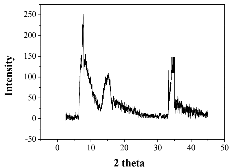
Figure S.2. X-ray diffraction data for aligned ODPA imogolite 30 times transferred at 0.5mN/m.
