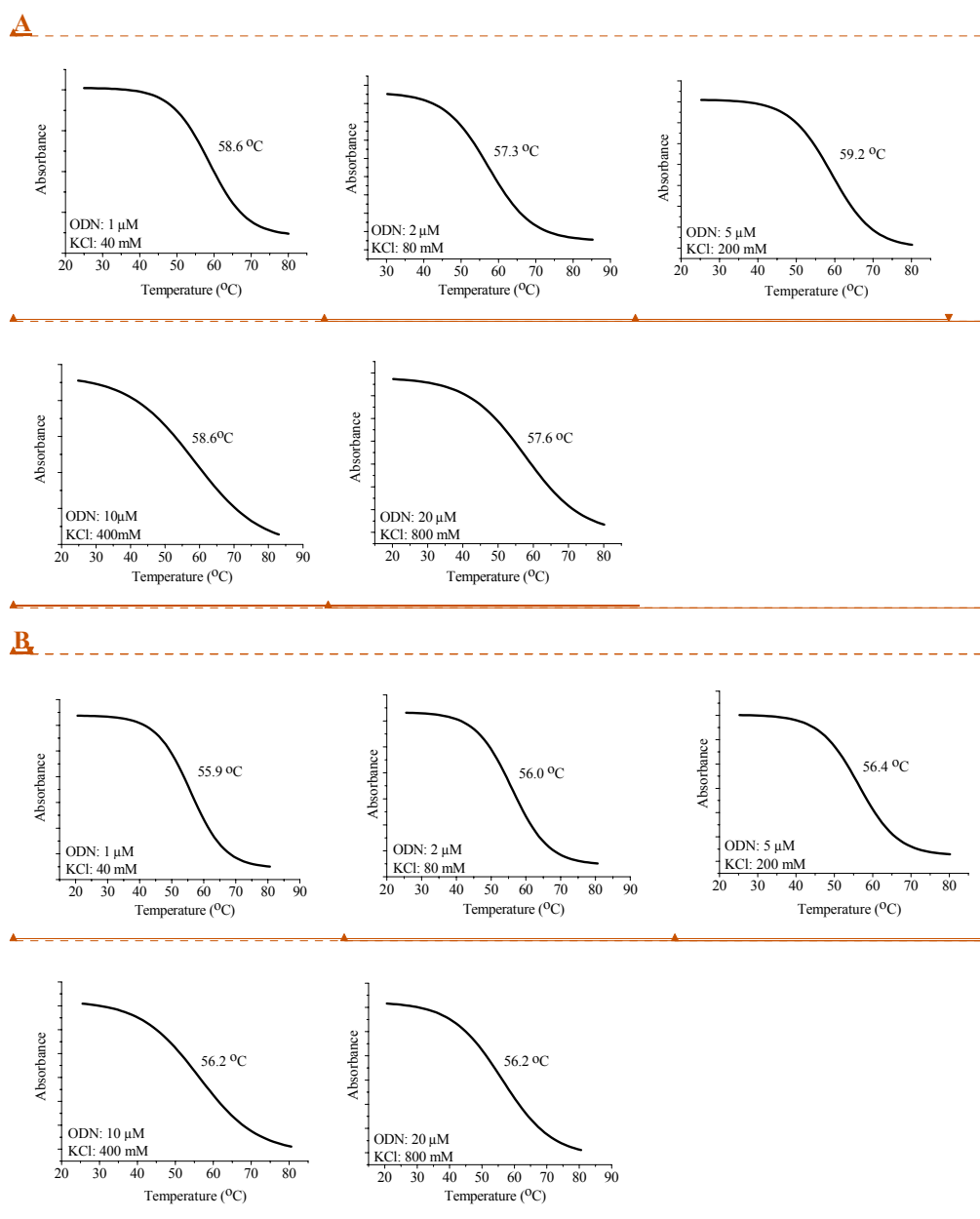
Figure S1. Melting temperature of (A) ODN S1 (B) ODN S3 with the diverse concentrations of KCl. All samples were prepared in 5 mM Tris-HCl buffer (pH 7.2), at 20 ^{\circ} C under irradiation at 295 nm.
