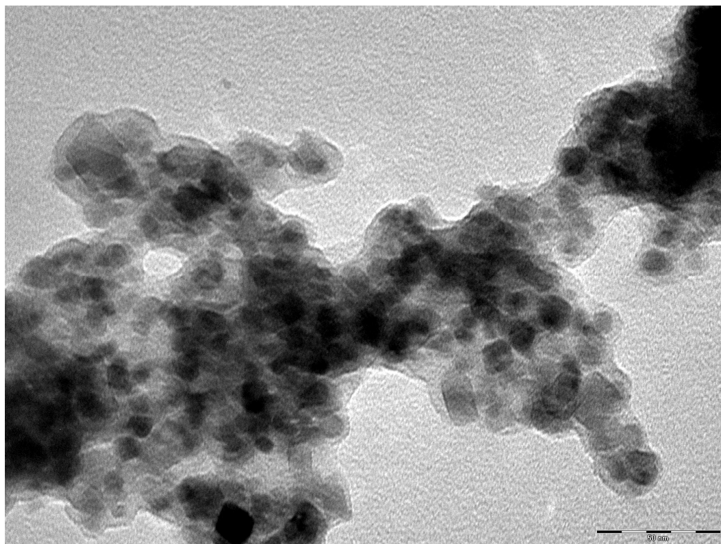
TEM images of the \gamma -Fe 2 O 3 nanoparticles after polymer functionalization.
