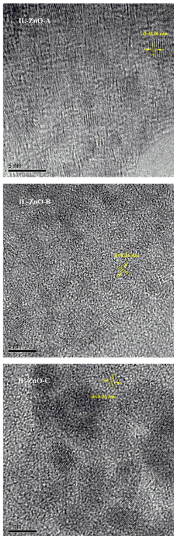
Figure S1 High-resolution TEM images of three samples (IL-ZnO-A, B and C). All of the images show a lattice plane spacing of 0.26 nm corresponding to the wurtzite structure.
