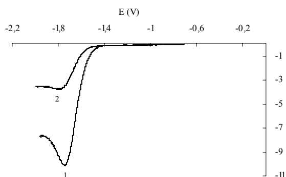
Fig. S1: Voltammograms recorded onto stainless steel for the reduction of NSA (0.1M) in DMF/5.10 -2 M TEAP, at 20 mV/s, (1) first scan and (2) second scan.
